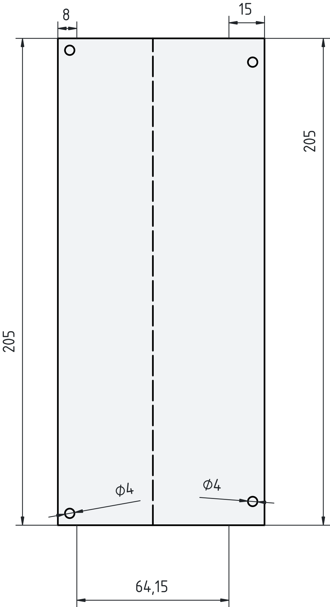
UNFOLD VIEW
